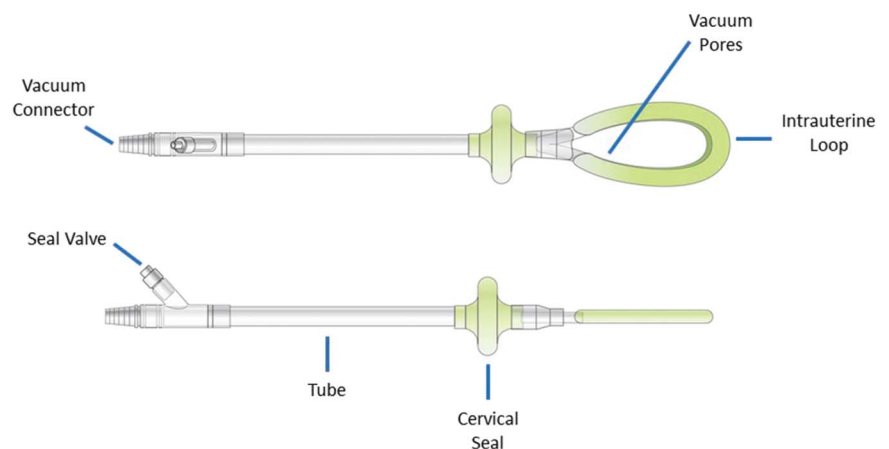
Fig. 1. The intrauterine vacuum-induced hemorrhage-control device (The Jada System). Image courtesy of Alydia Health. Used with permission.
